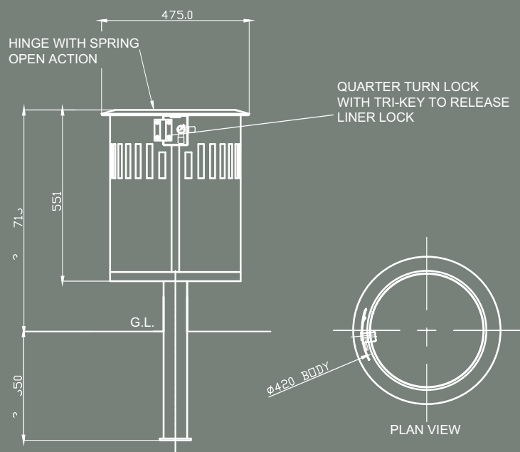
SPIGOT MOUNTED TYPE FRONT ELEVATION
