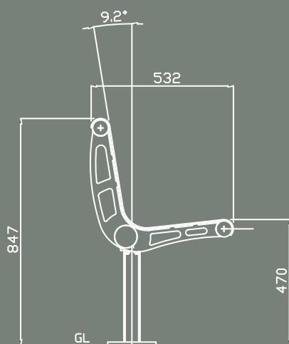
TYPICAL ELEVATION
