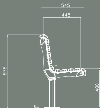
TYPICAL ELEVATION
