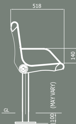
SUB-SURFACE MOUNTED TYPE TYPICAL ELEVATION WITH FLORENTINE ARM
