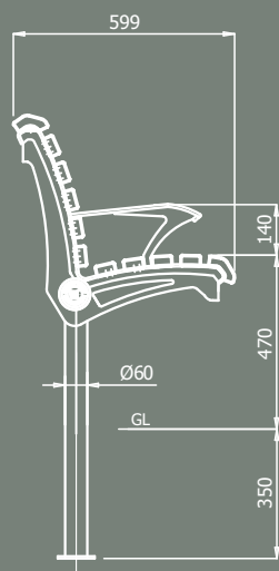
SPIGOT MOUNTED TYPE TYPICAL ELEVATION WITH ARMREST
