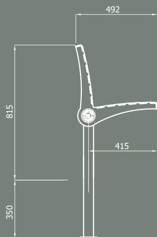
SPIGOT MOUNTED TYPE TYPICAL ELEVATION
