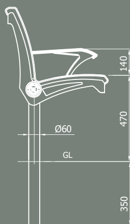
SPIGOT MOUNTED TYPE TYPICAL ELEVATION WITH ARMREST
