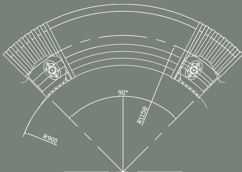
PLAN - STRAPS REMOVED FOR CLARITY
