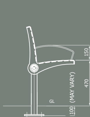
SUB-SURFACE MOUNTED TYPE TYPICAL ELEVATION WITH MANNHEIM ARM
